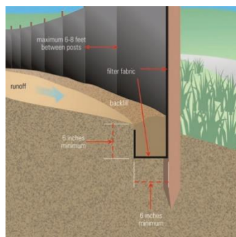
SILT FENCE
