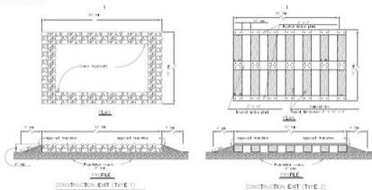
1. Construction Entrance
